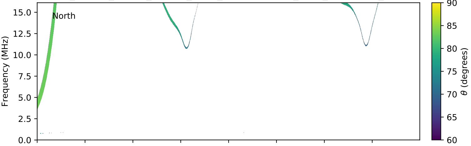
expres_cassini_jupiter_europa_isaac_lossc-wid1deg_3kev_20010901_v01.cdf
