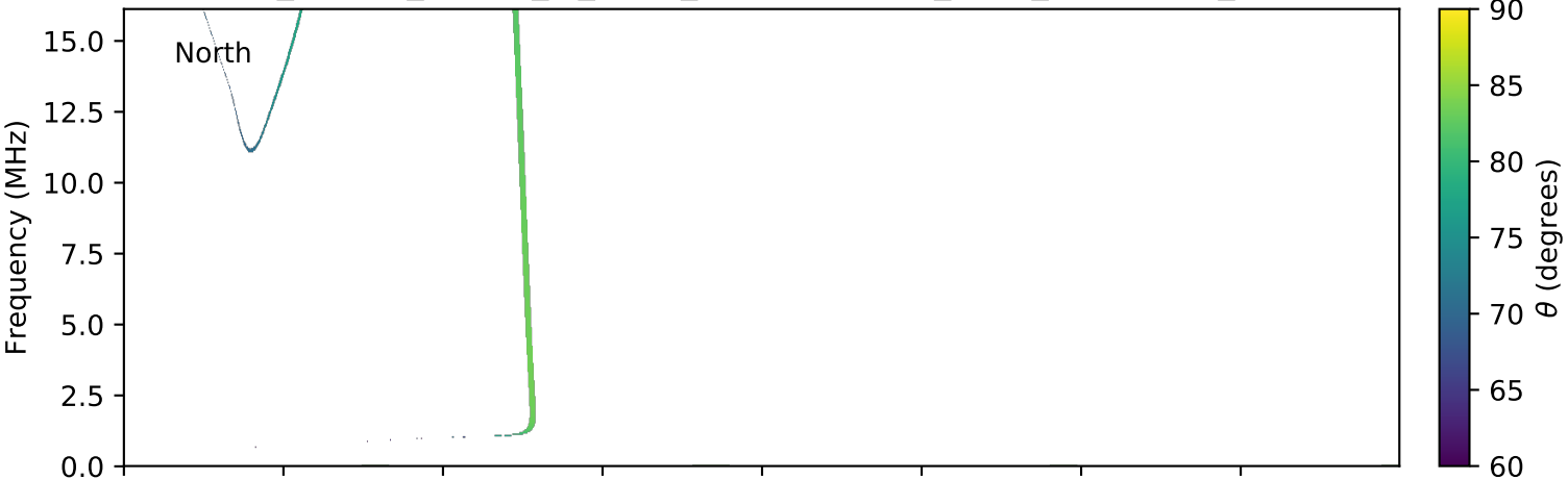
expres_cassini_jupiter_io_isaac_lossc-wid1deg_3kev_20010827_v01.cdf
