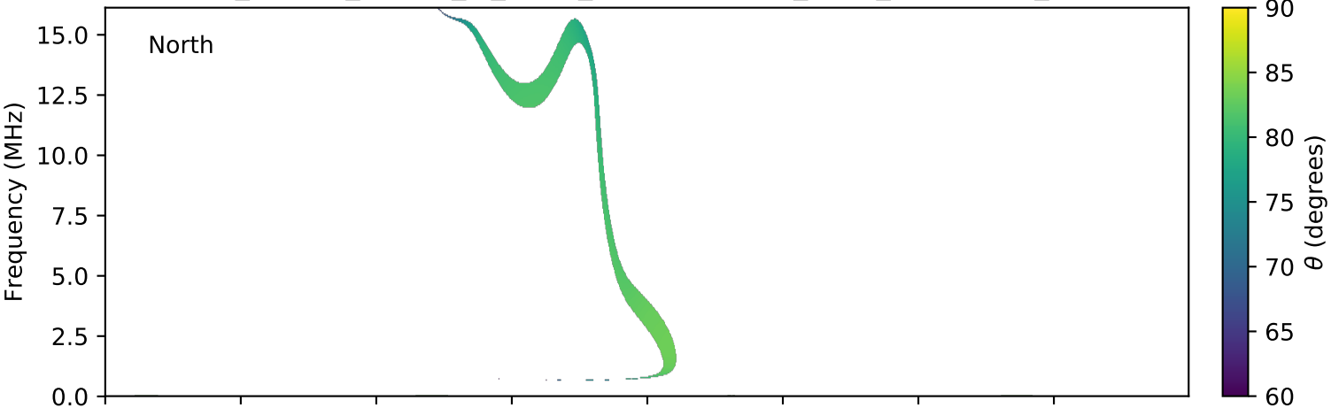
expres_cassini_jupiter_io_isaac_lossc-wid1deg_3kev_20010825_v01.cdf
