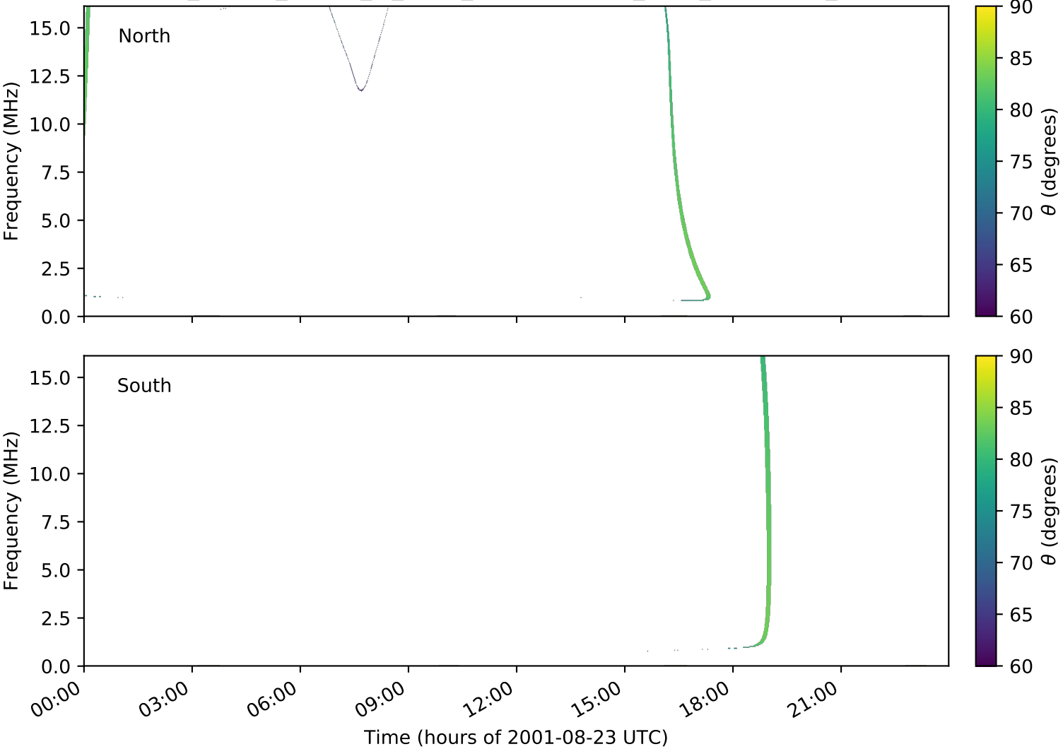
expres_cassini_jupiter_io_isaac_lossc-wid1deg_3kev_20010823_v01.cdf
