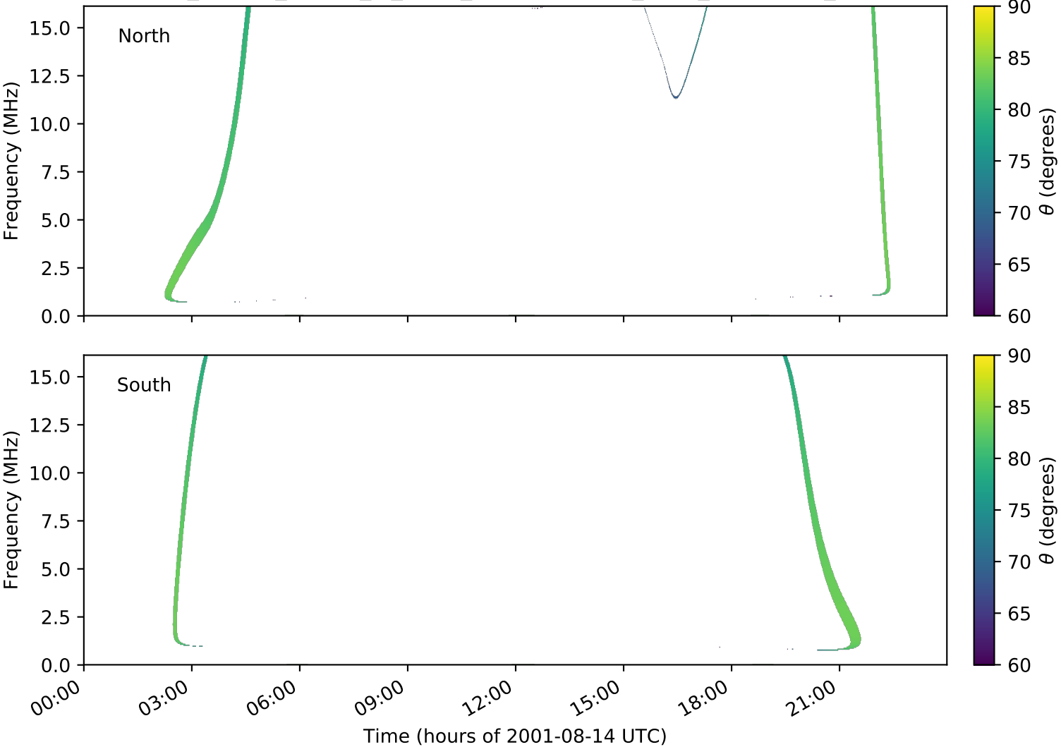
expres_cassini_jupiter_io_isaac_lossc-wid1deg_3kev_20010814_v01.cdf
