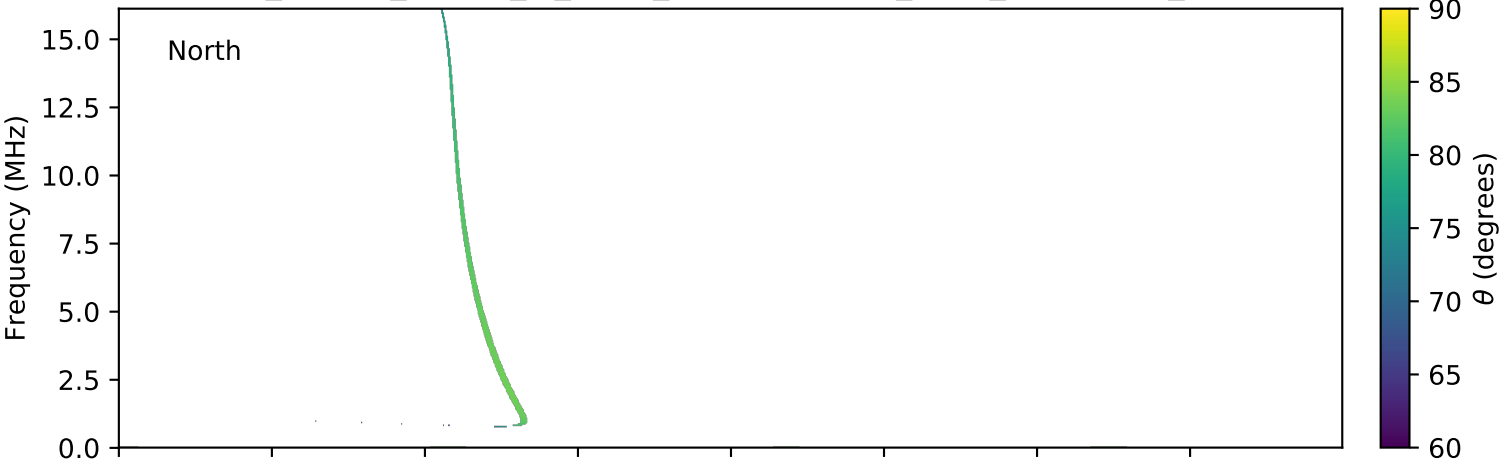
expres_cassini_jupiter_io_isaac_lossc-wid1deg_3kev_20010811_v01.cdf
