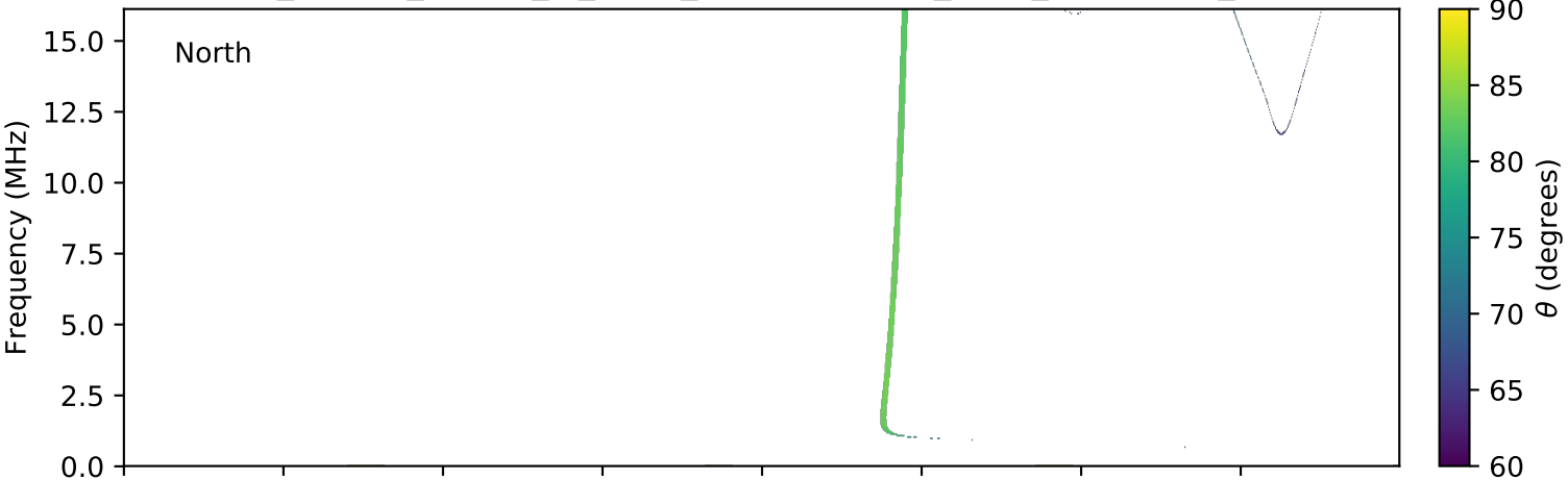
expres_cassini_jupiter_io_isaac_lossc-wid1deg_3kev_20010810_v01.cdf
