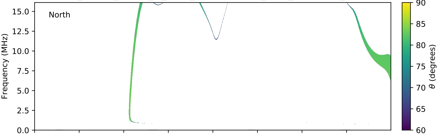
expres_cassini_jupiter_io_isaac_lossc-wid1deg_3kev_20010805_v01.cdf
