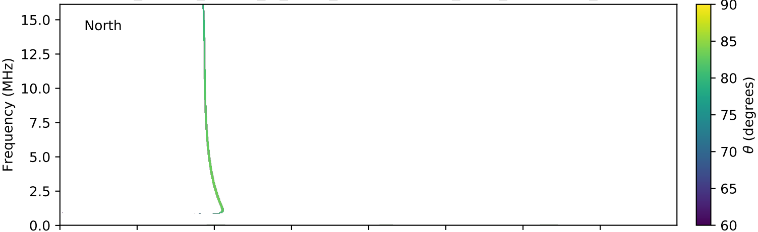
expres_cassini_jupiter_io_isaac_lossc-wid1deg_3kev_20010804_v01.cdf
