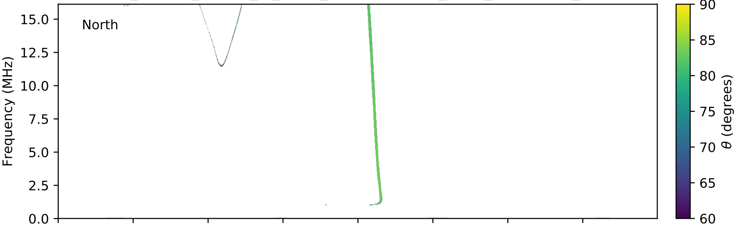
expres_cassini_jupiter_io_isaac_lossc-wid1deg_3kev_20010802_v01.cdf
