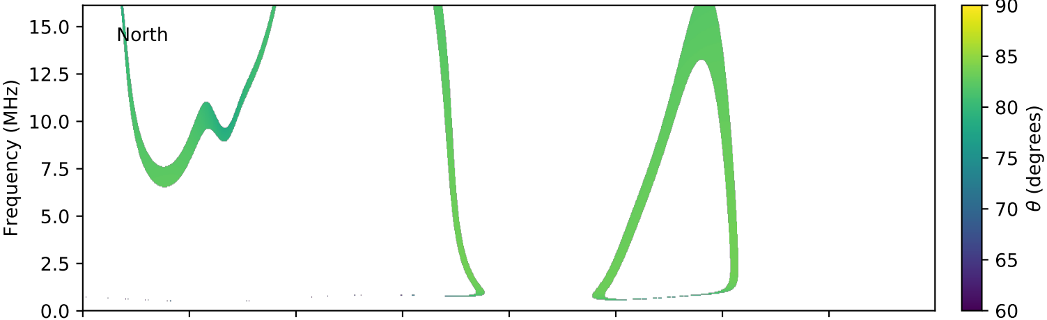
expres_cassini_jupiter_ganymede_isaac_lossc-wid1deg_3kev_20010829_v01.cdf
