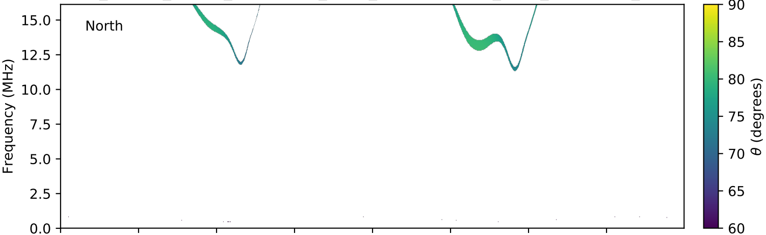
expres_cassini_jupiter_ganymede_isaac_lossc-wid1deg_3kev_20010828_v01.cdf
