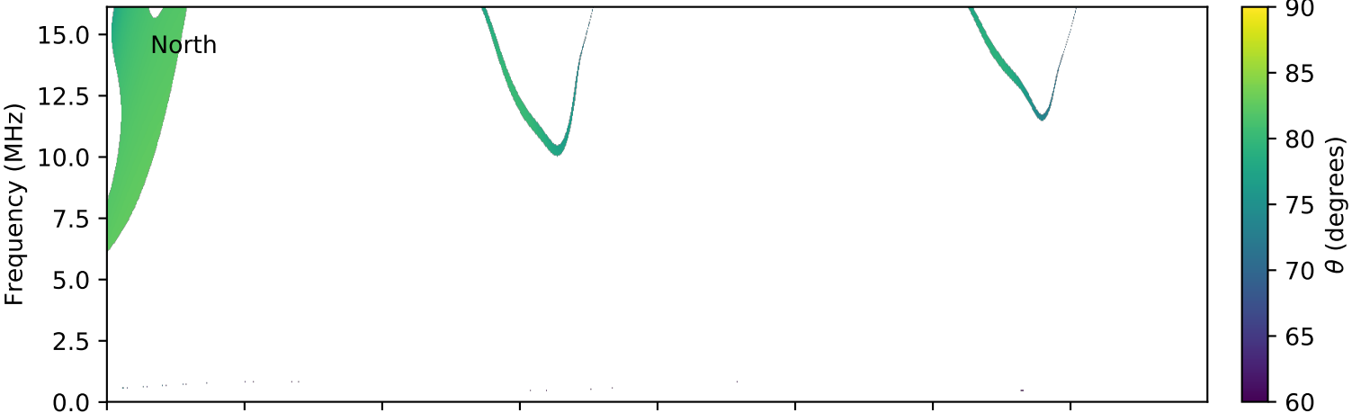
expres_cassini_jupiter_ganymede_isaac_lossc-wid1deg_3kev_20010827_v01.cdf
