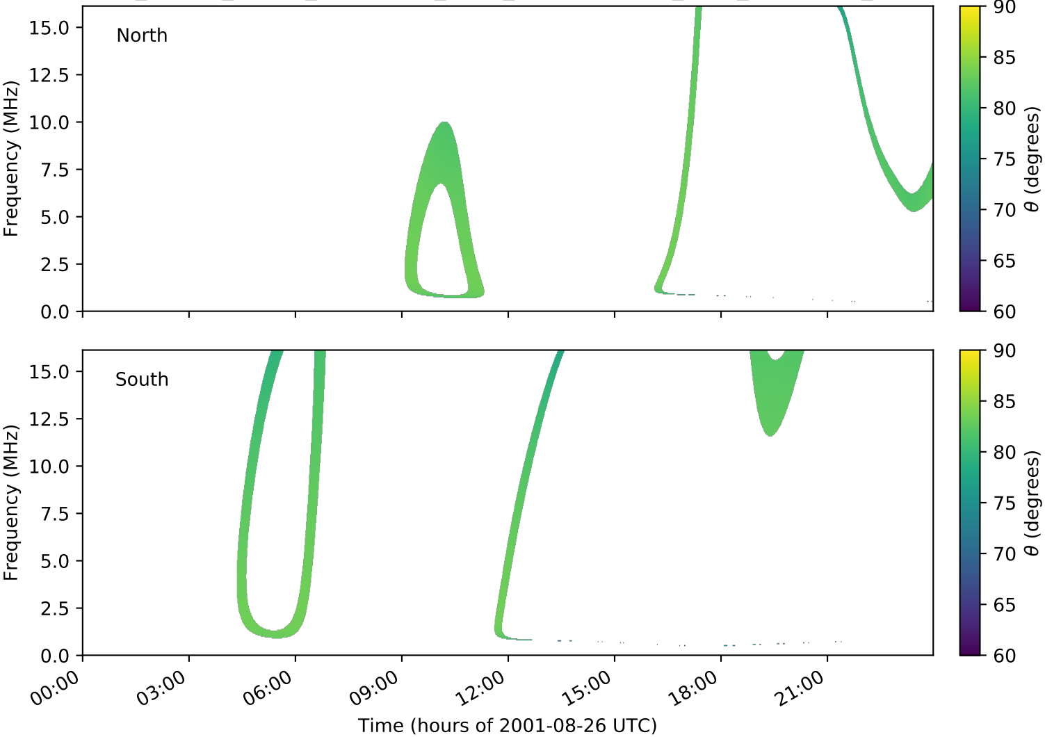
expres_cassini_jupiter_ganymede_isaac_lossc-wid1deg_3kev_20010826_v01.cdf
