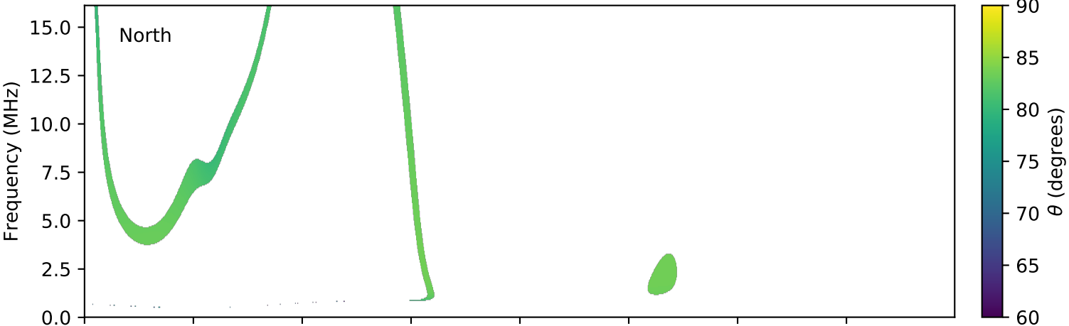
expres_cassini_jupiter_ganymede_isaac_lossc-wid1deg_3kev_20010822_v01.cdf
