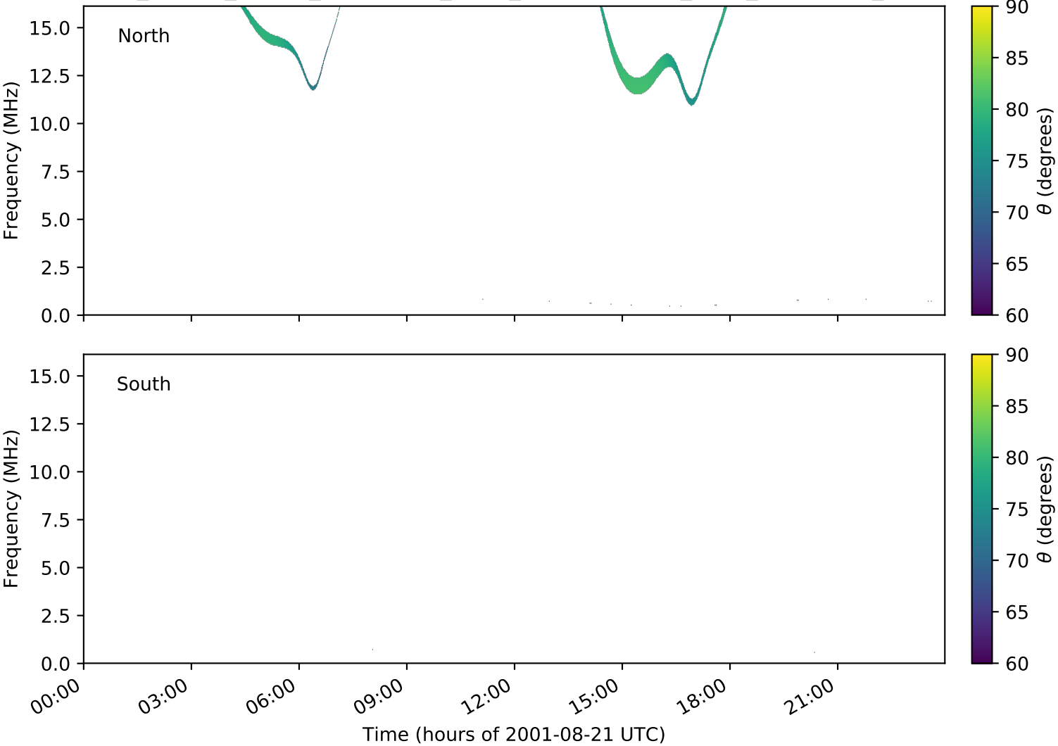
expres_cassini_jupiter_ganymede_isaac_lossc-wid1deg_3kev_20010821_v01.cdf
