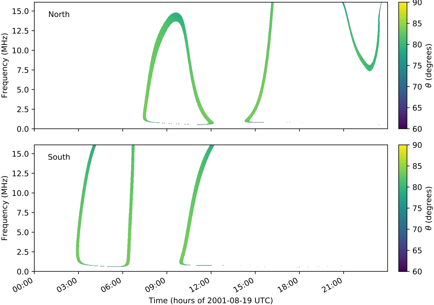
expres_cassini_jupiter_ganymede_isaac_lossc-wid1deg_3kev_20010819_v01.cdf
