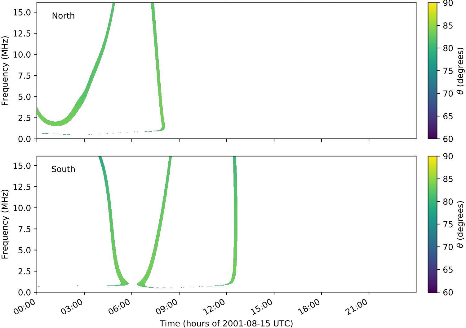
expres_cassini_jupiter_ganymede_isaac_lossc-wid1deg_3kev_20010815_v01.cdf
