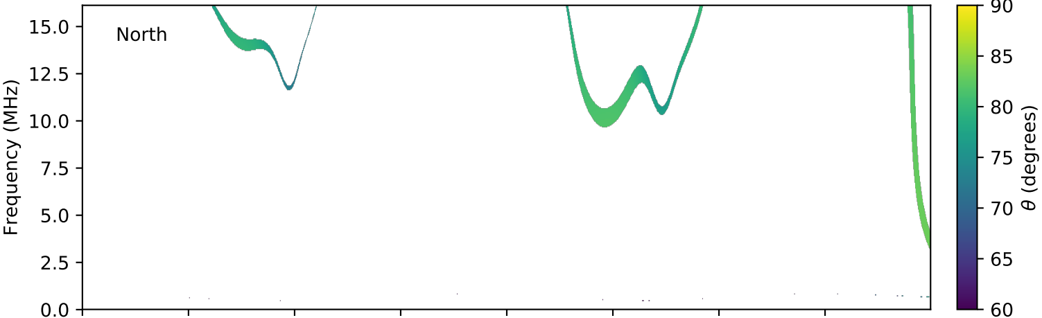
expres_cassini_jupiter_ganymede_isaac_lossc-wid1deg_3kev_20010814_v01.cdf
