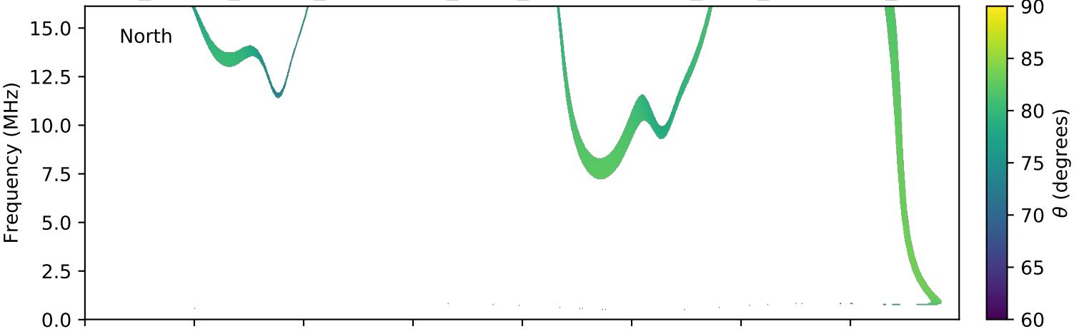
expres_cassini_jupiter_ganymede_isaac_lossc-wid1deg_3kev_20010807_v01.cdf
