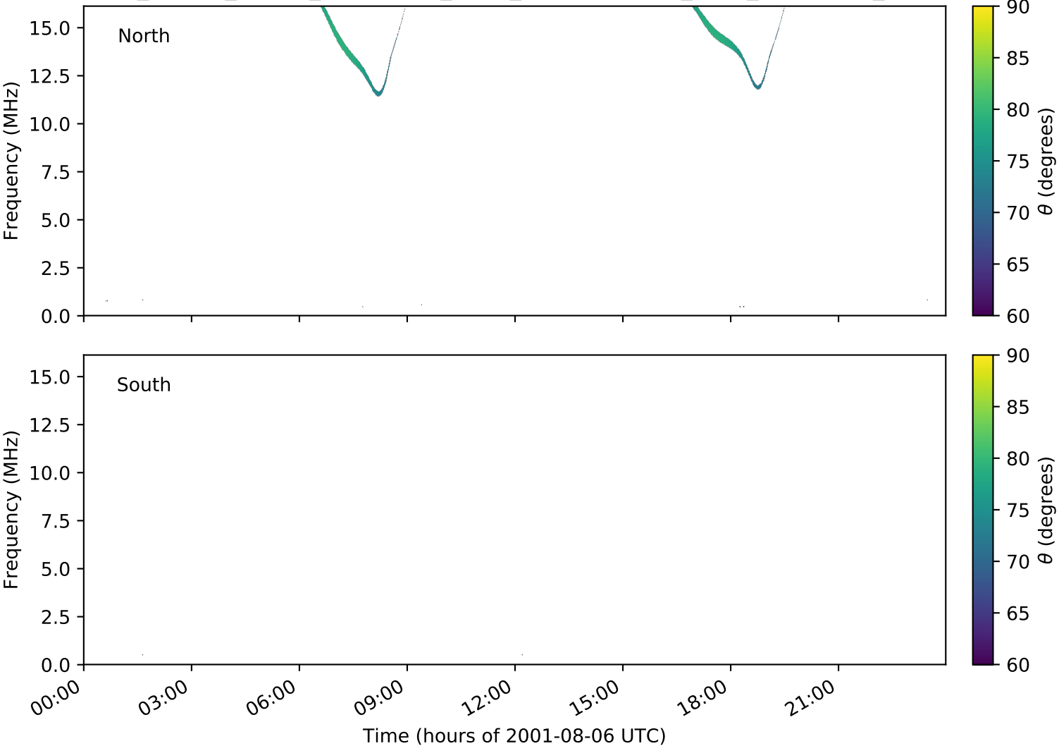
expres_cassini_jupiter_ganymede_isaac_lossc-wid1deg_3kev_20010806_v01.cdf
