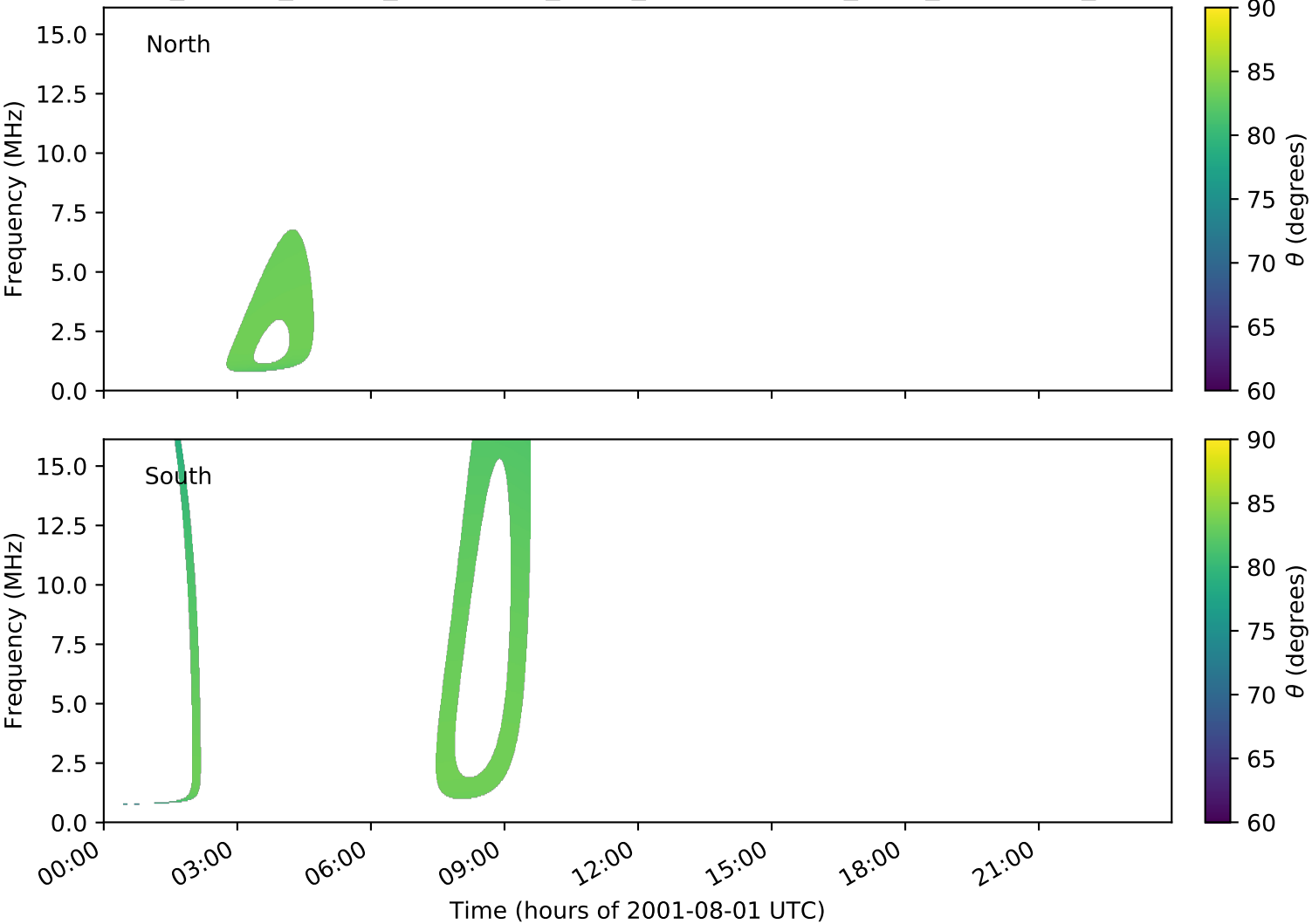
expres_cassini_jupiter_ganymede_isaac_lossc-wid1deg_3kev_20010801_v01.cdf
