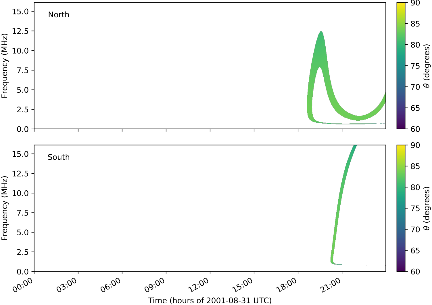
expres_cassini_jupiter_europa_isaac_lossc-wid1deg_3kev_20010831_v01.cdf
