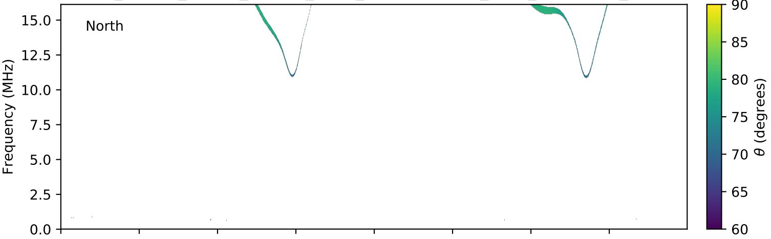
expres_cassini_jupiter_europa_isaac_lossc-wid1deg_3kev_20010825_v01.cdf
