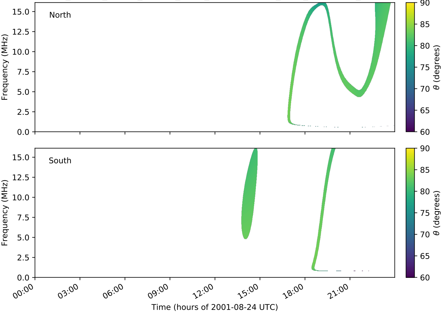
expres_cassini_jupiter_europa_isaac_lossc-wid1deg_3kev_20010824_v01.cdf
