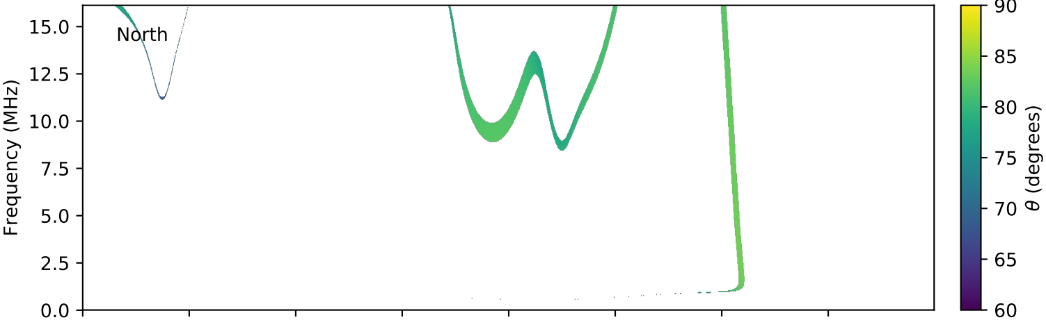
expres_cassini_jupiter_europa_isaac_lossc-wid1deg_3kev_20010822_v01.cdf
