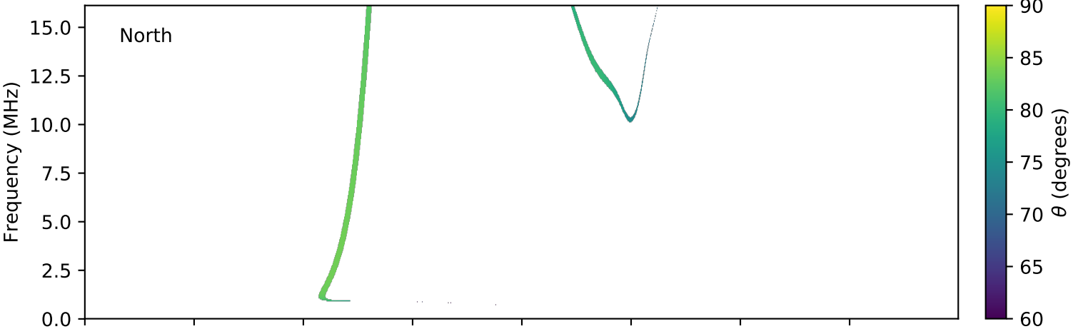
expres_cassini_jupiter_europa_isaac_lossc-wid1deg_3kev_20010821_v01.cdf
