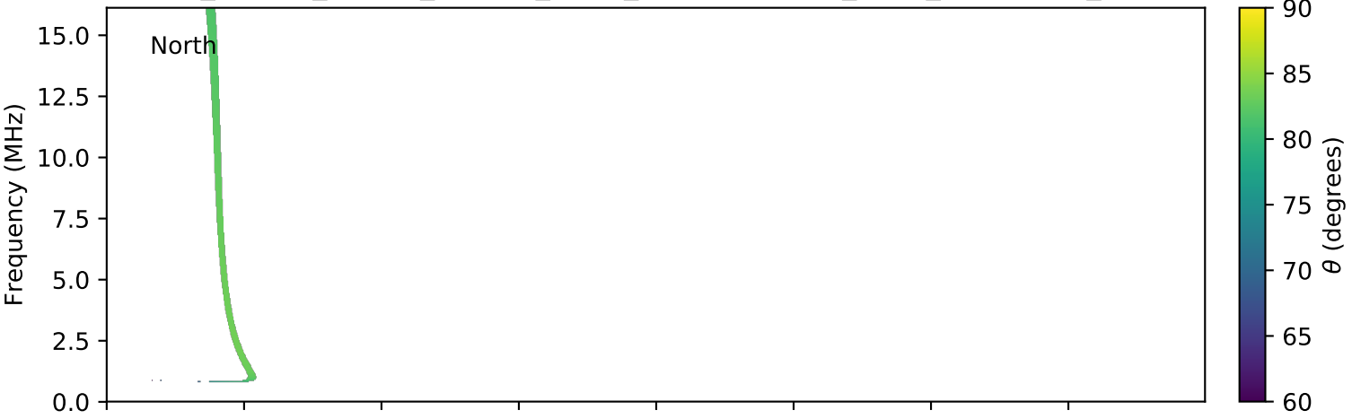
expres_cassini_jupiter_europa_isaac_lossc-wid1deg_3kev_20010819_v01.cdf
