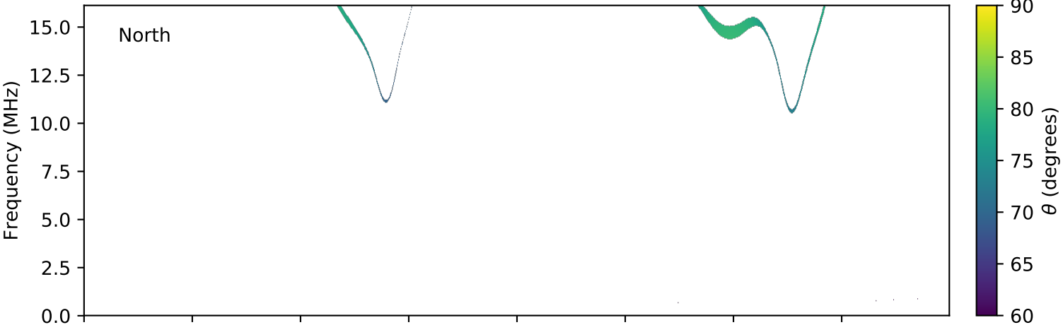
expres_cassini_jupiter_europa_isaac_lossc-wid1deg_3kev_20010818_v01.cdf
