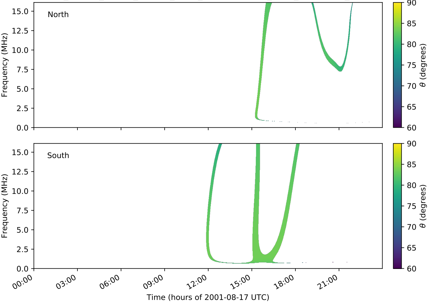
expres_cassini_jupiter_europa_isaac_lossc-wid1deg_3kev_20010817_v01.cdf
