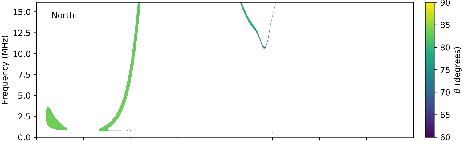
expres_cassini_jupiter_europa_isaac_lossc-wid1deg_3kev_20010814_v01.cdf
