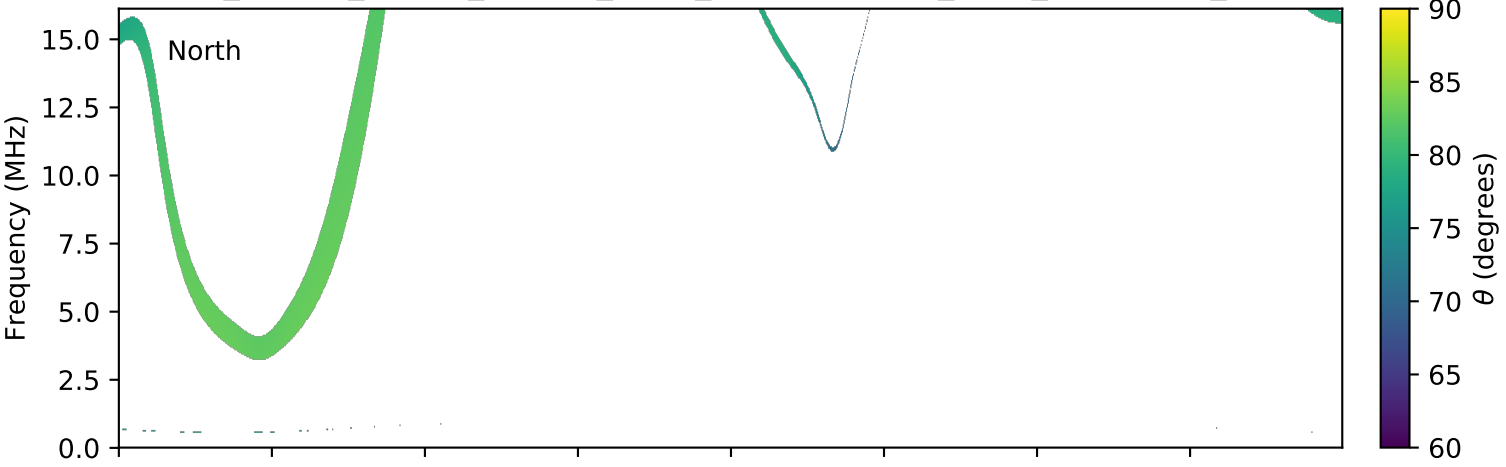
expres_cassini_jupiter_europa_isaac_lossc-wid1deg_3kev_20010807_v01.cdf
