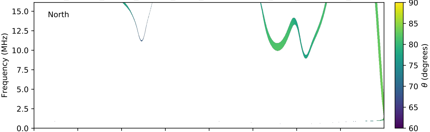
expres_cassini_jupiter_europa_isaac_lossc-wid1deg_3kev_20010804_v01.cdf
