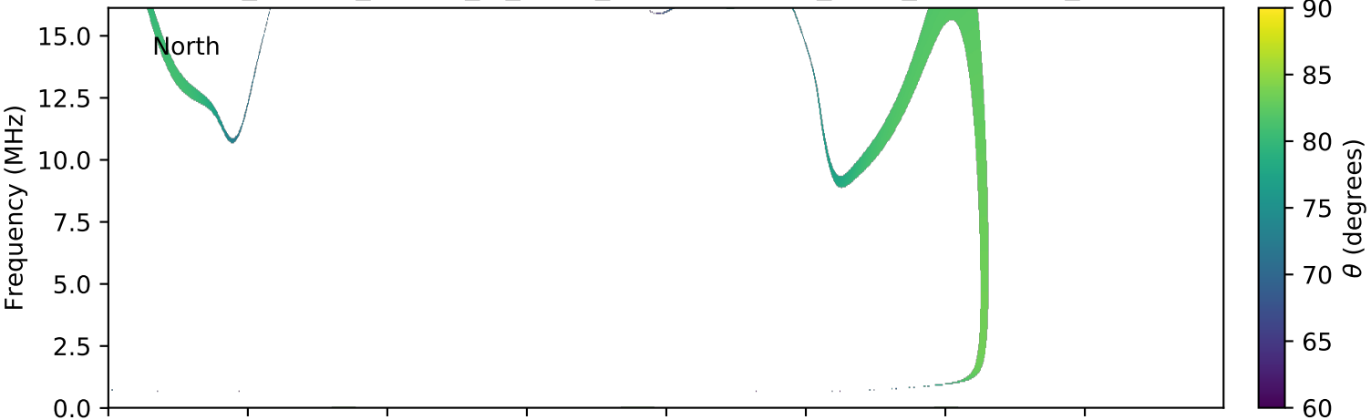
expres_cassini_jupiter_io_isaac_lossc-wid1deg_3kev_20010731_v01.cdf
