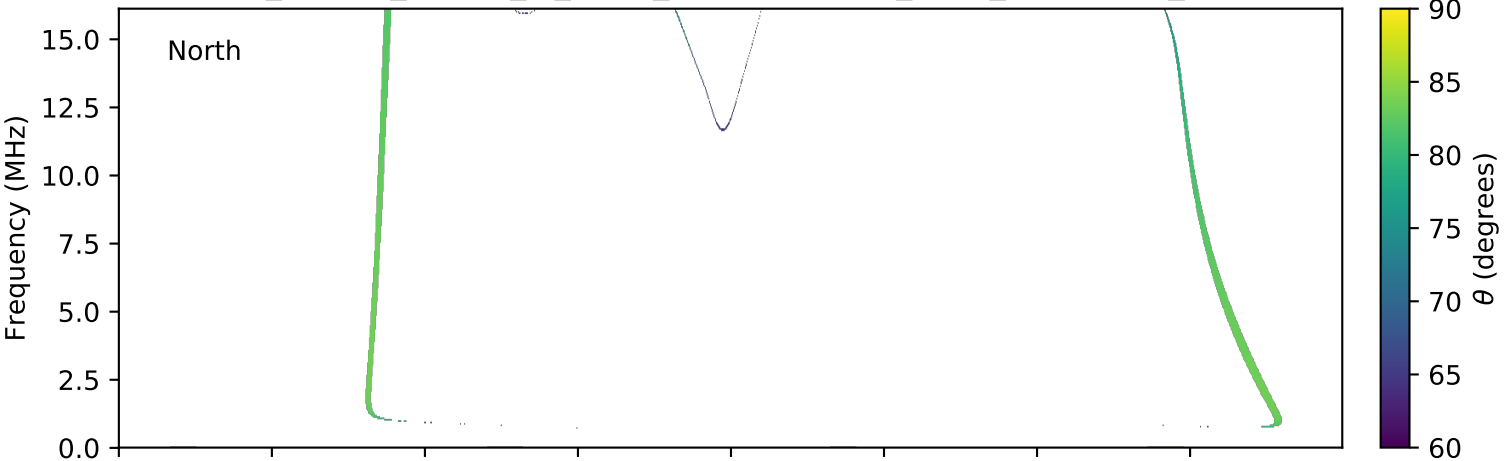
expres_cassini_jupiter_io_isaac_lossc-wid1deg_3kev_20010729_v01.cdf
