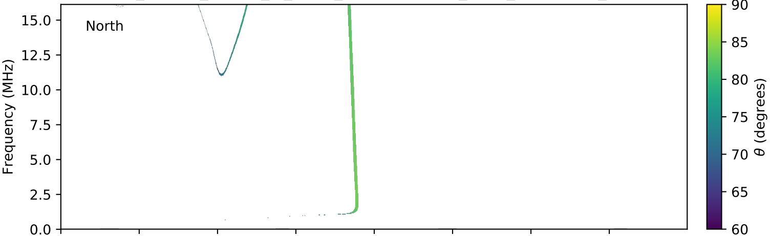
expres_cassini_jupiter_io_isaac_lossc-wid1deg_3kev_20010726_v01.cdf
