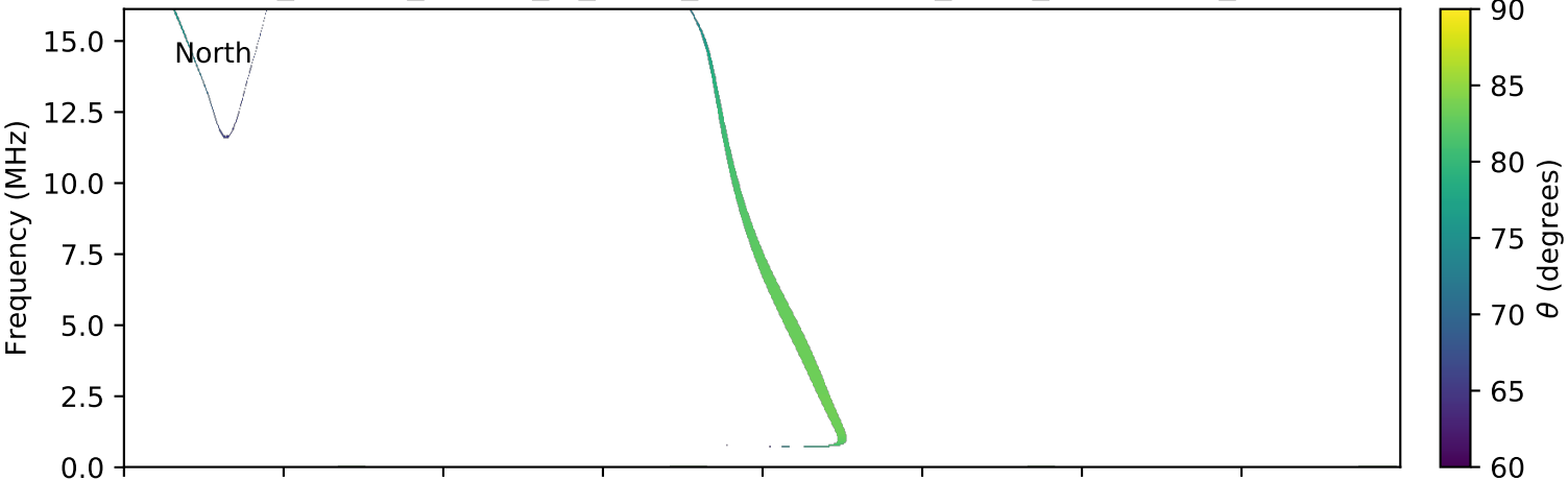
expres_cassini_jupiter_io_isaac_lossc-wid1deg_3kev_20010717_v01.cdf
