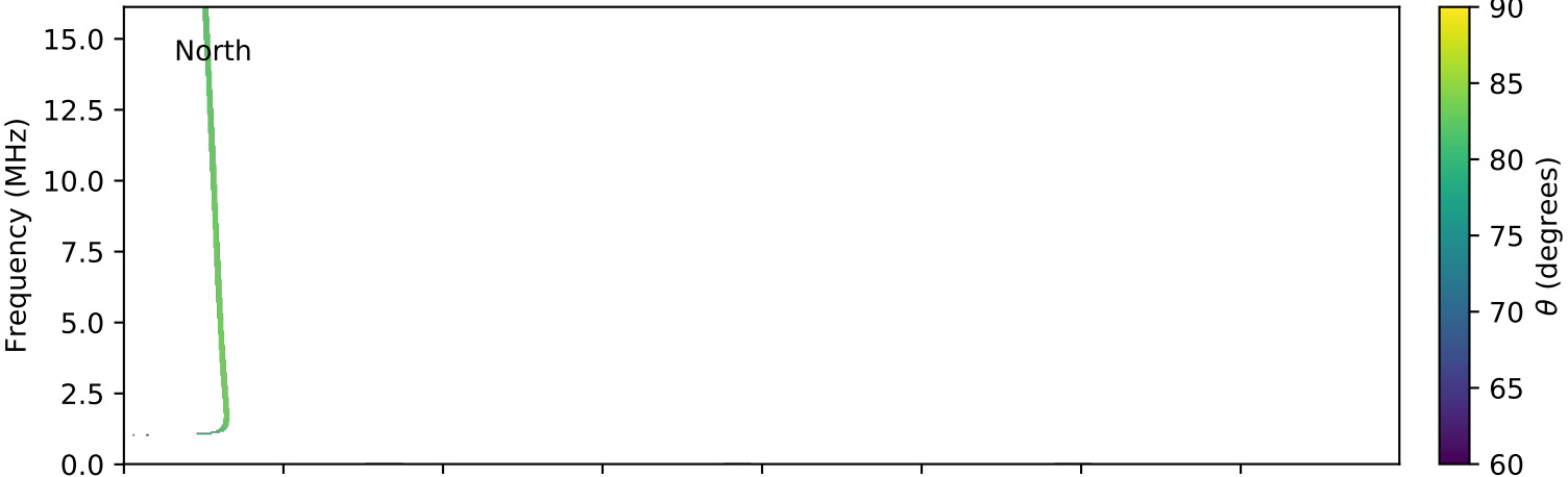
expres_cassini_jupiter_io_isaac_lossc-wid1deg_3kev_20010714_v01.cdf
