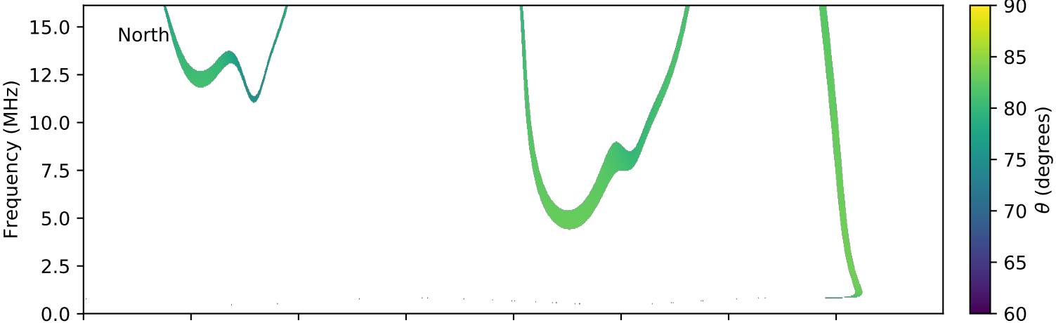
expres_cassini_jupiter_ganymede_isaac_lossc-wid1deg_3kev_20010731_v01.cdf
