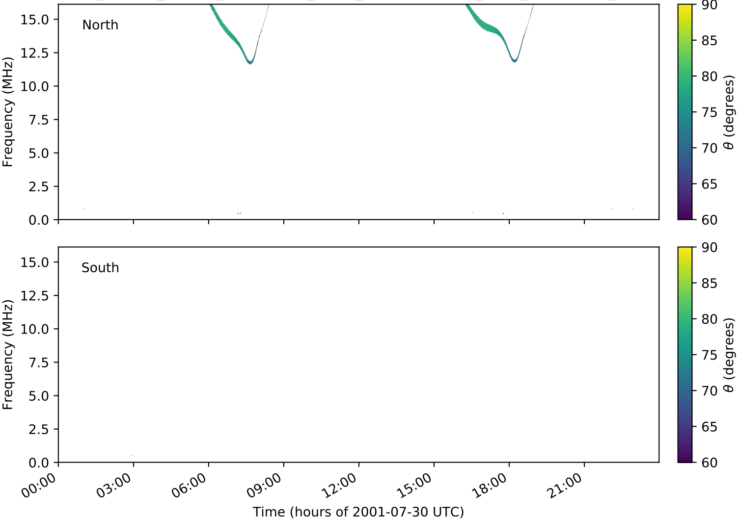
expres_cassini_jupiter_ganymede_isaac_lossc-wid1deg_3kev_20010730_v01.cdf
