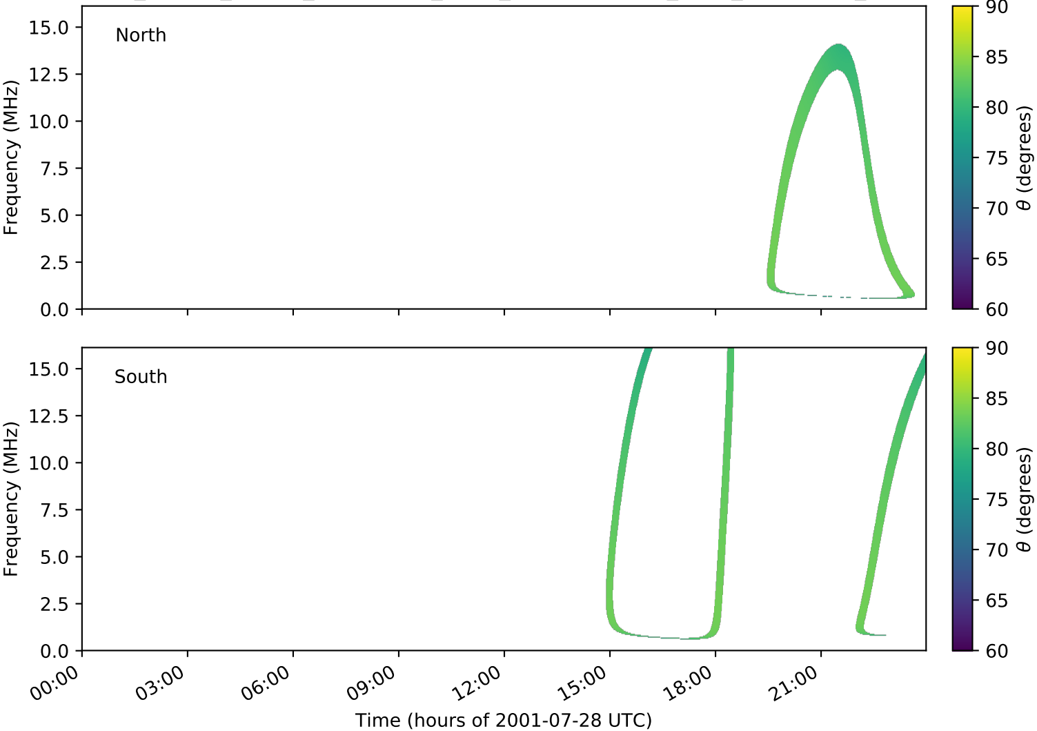
expres_cassini_jupiter_ganymede_isaac_lossc-wid1deg_3kev_20010728_v01.cdf
