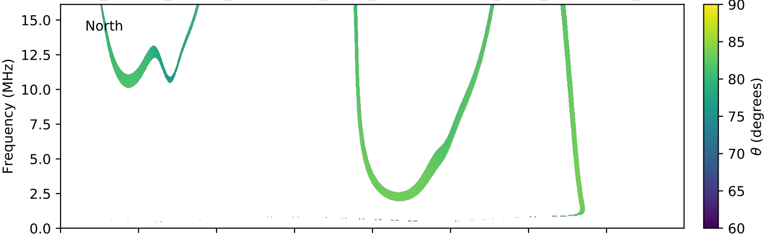
expres_cassini_jupiter_ganymede_isaac_lossc-wid1deg_3kev_20010724_v01.cdf
