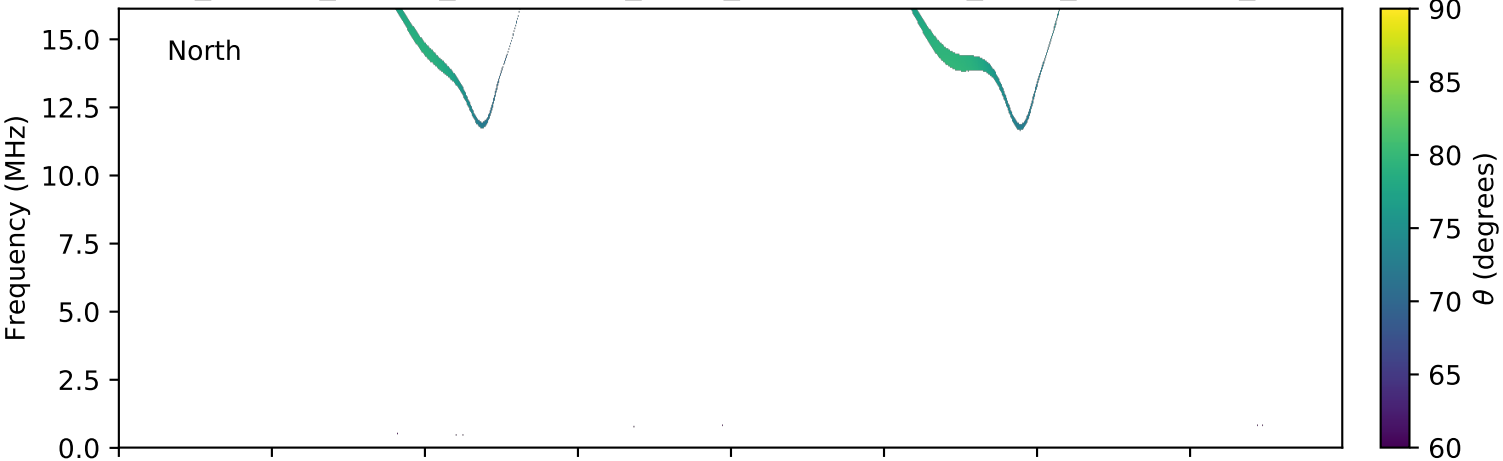
expres_cassini_jupiter_ganymede_isaac_lossc-wid1deg_3kev_20010723_v01.cdf
