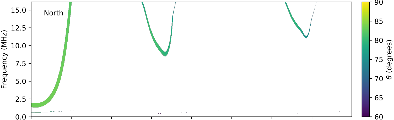
expres_cassini_jupiter_ganymede_isaac_lossc-wid1deg_3kev_20010722_v01.cdf
