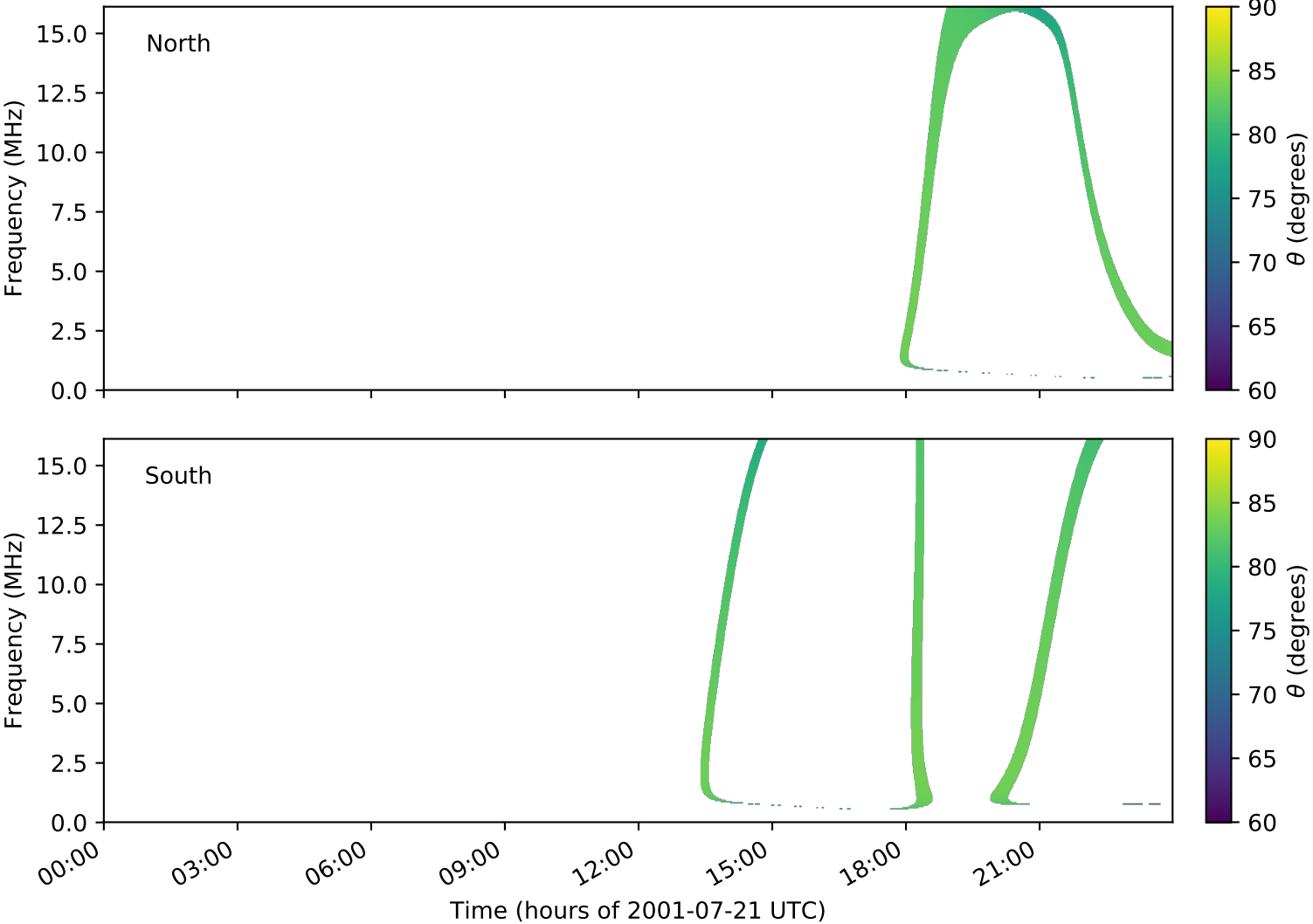
expres_cassini_jupiter_ganymede_isaac_lossc-wid1deg_3kev_20010721_v01.cdf
