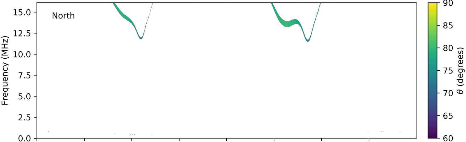
expres_cassini_jupiter_ganymede_isaac_lossc-wid1deg_3kev_20010716_v01.cdf
