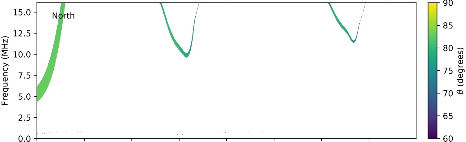
expres_cassini_jupiter_ganymede_isaac_lossc-wid1deg_3kev_20010715_v01.cdf
