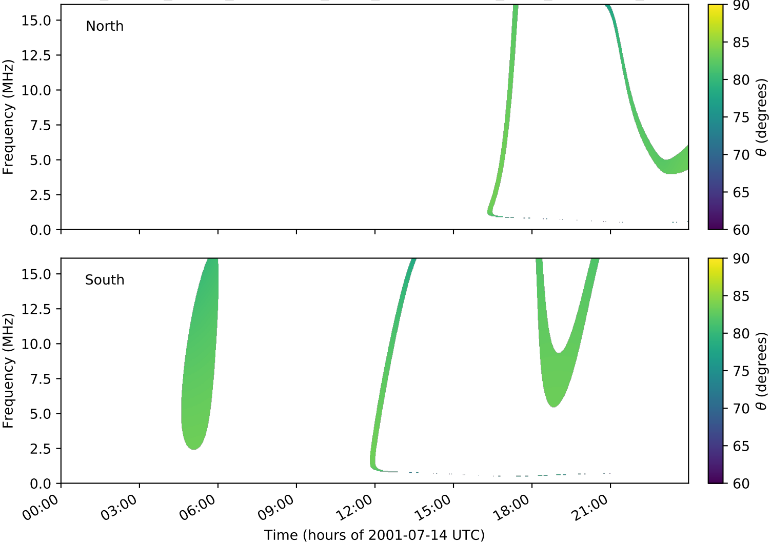
expres_cassini_jupiter_ganymede_isaac_lossc-wid1deg_3kev_20010714_v01.cdf
