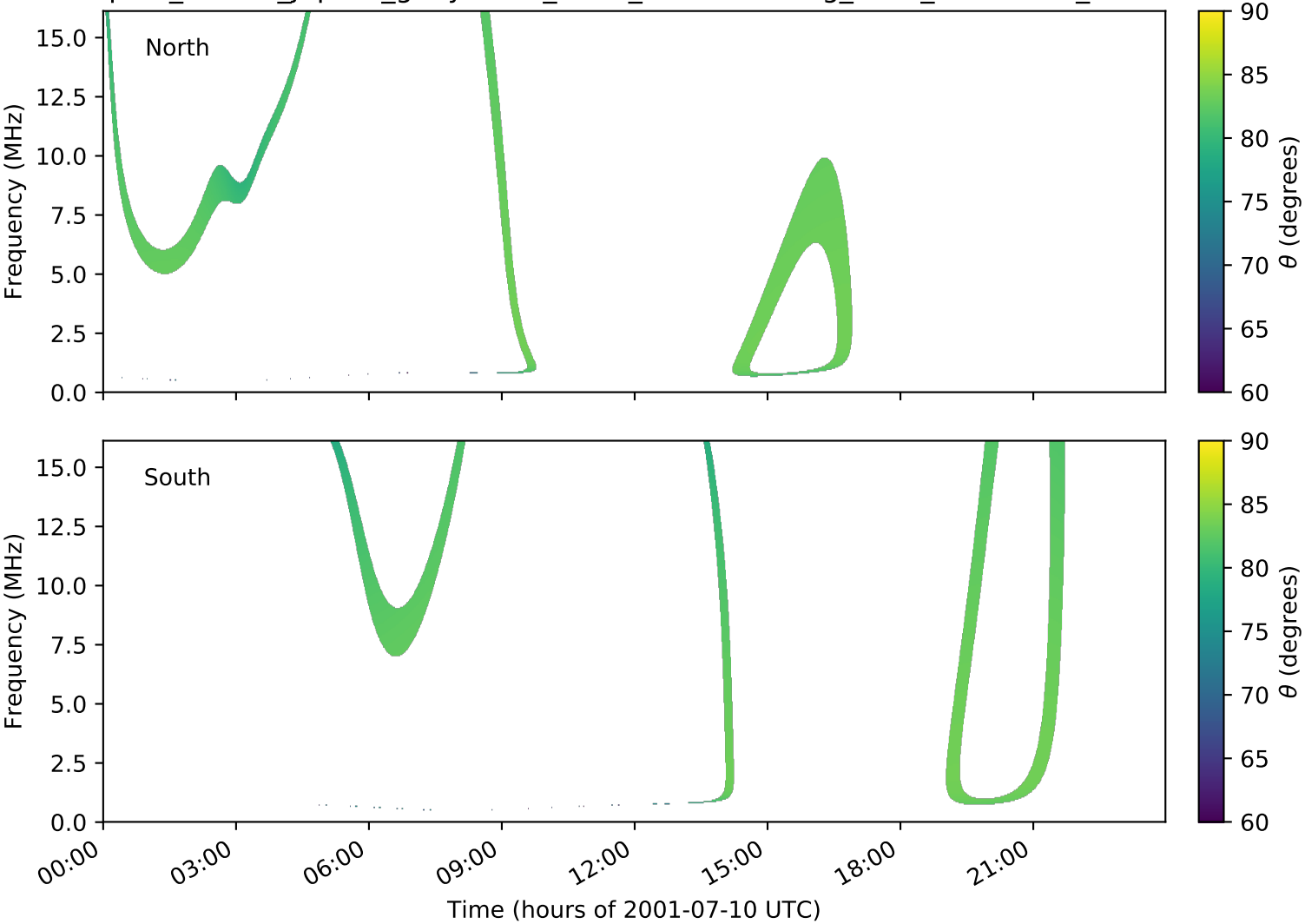
expres_cassini_jupiter_ganymede_isaac_lossc-wid1deg_3kev_20010710_v01.cdf
