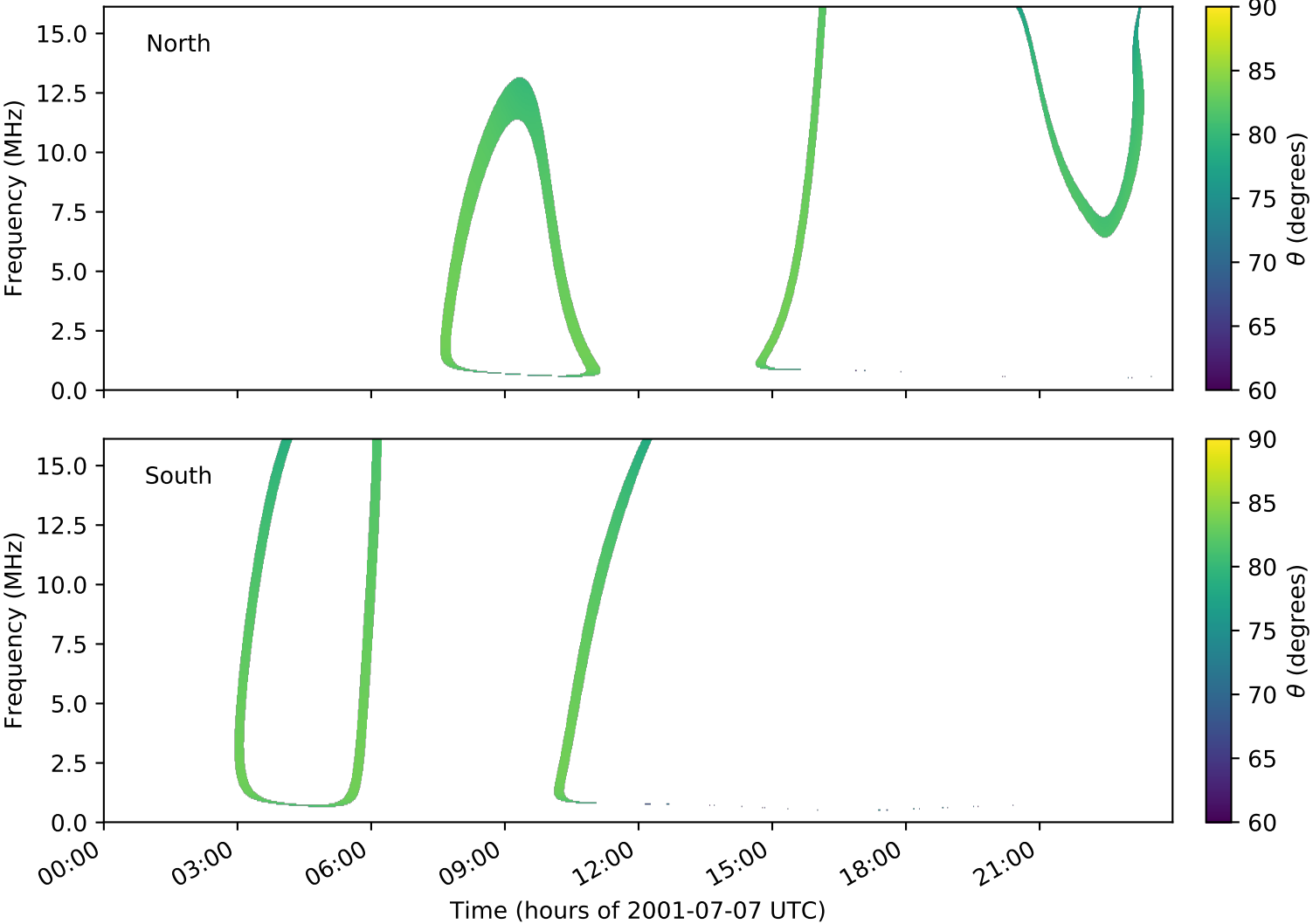
expres_cassini_jupiter_ganymede_isaac_lossc-wid1deg_3kev_20010707_v01.cdf
